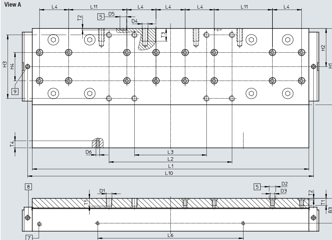
View A
