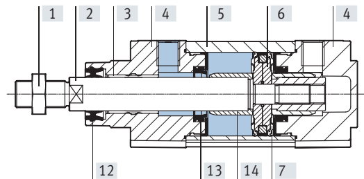
Sectional view – Basic design
