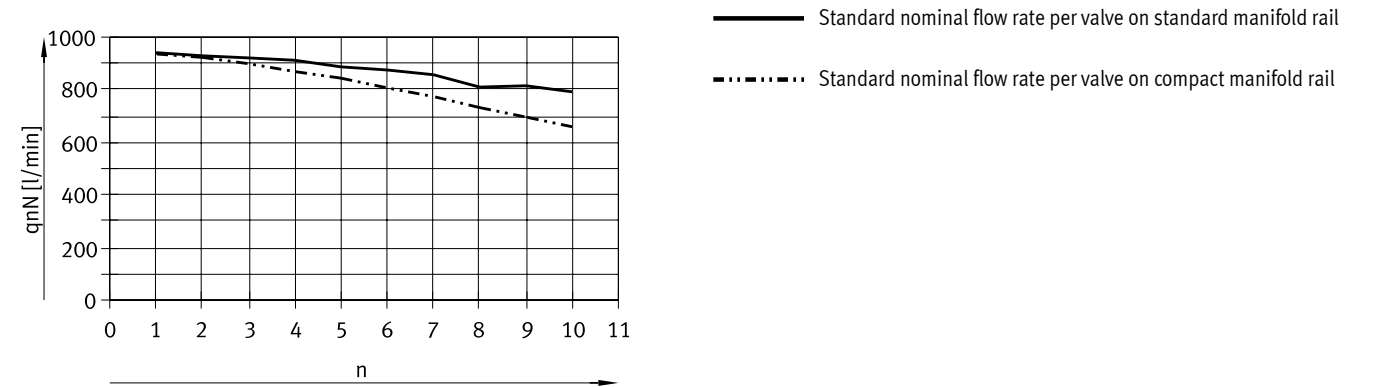
Size 25 – Standard nominal flow rate q_{nN} , with several valves n switched in parallel For 2x 3/2-way valves One valve function per valve position in open switching position
