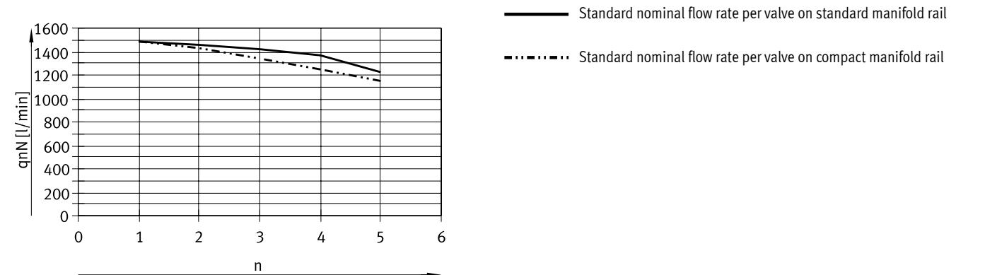
For 2x 3/2-way valves Both valve functions per valve position simultaneously in open switching position
