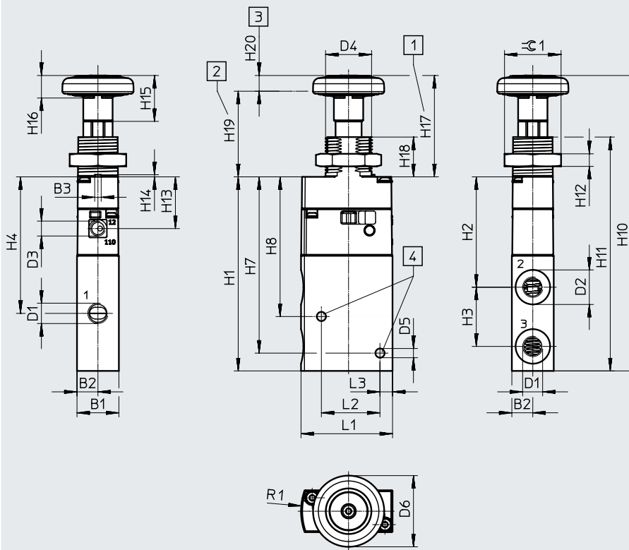
[1] Normal position
