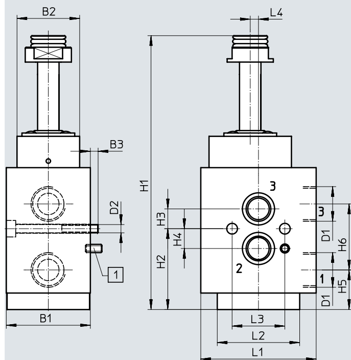
[1] Coding pin M5x10
