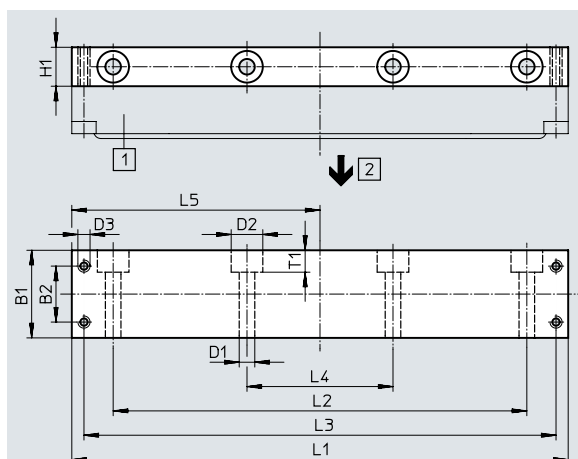
[1] Clamping module EV [2] Clamping direction
