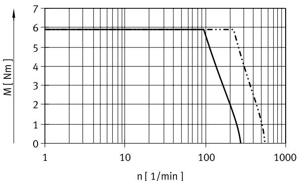
Torque M as a function of rotational speed n EMMS-ST-87-S
