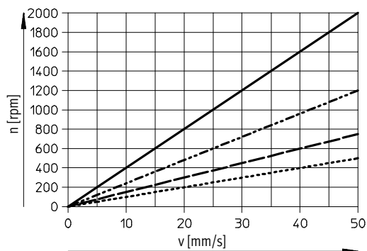
Speed as a function of the feed speed v
