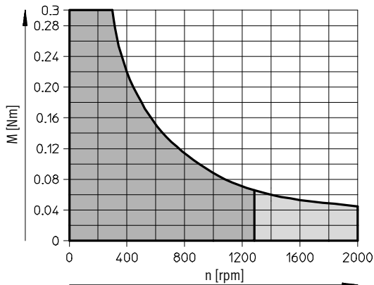
Maximum permissible driving torque M as a function of n (rpm)
