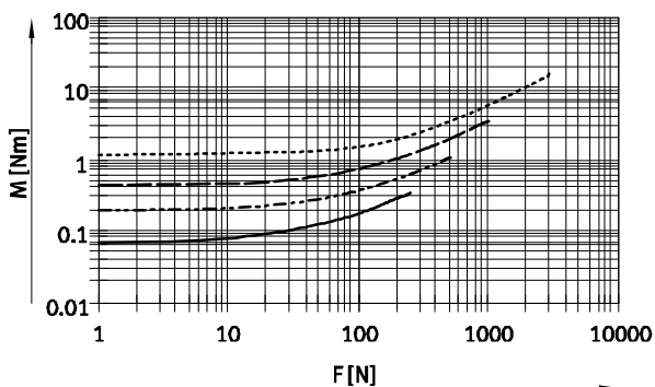
Driving torque M as a function of the feed force F
