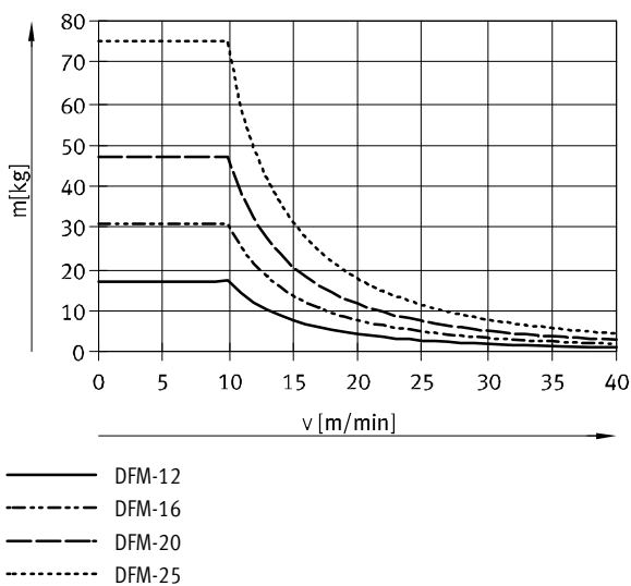
DFM-12 ... 25-GF, stroke < 30 mm
