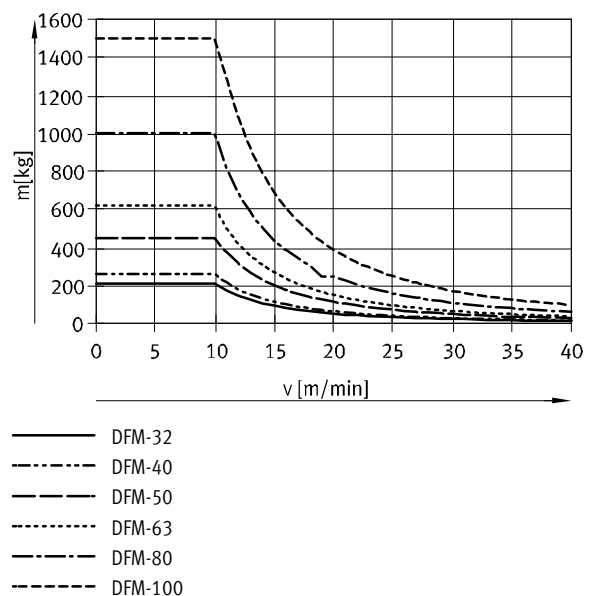
DFM-32 ... 100-GF, stroke < 50 mm
