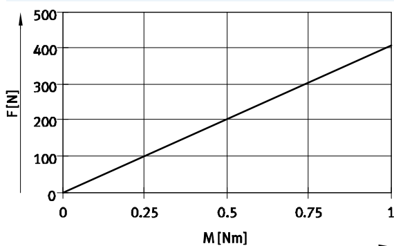
Theoretical feed force F as a function of input torque M
