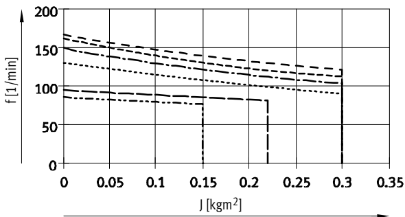
Max. permissible cycle frequency f as a function of mass moment of inertia J
