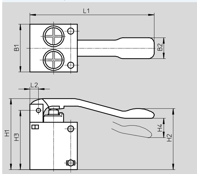
Tasthebelventil TH-5-1/4-B
