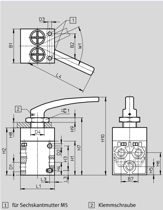
Handhebelventil H-5-¼-B
