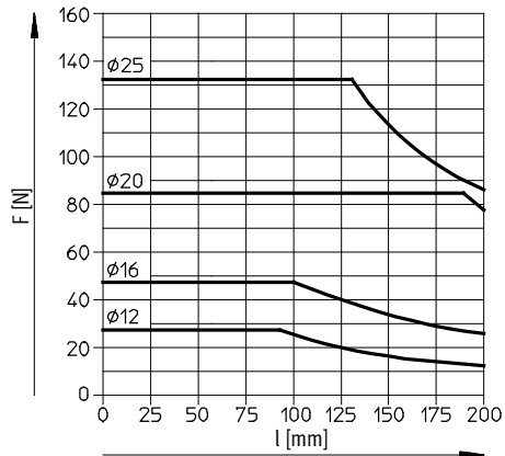
DFM-12 ... 25-GF Carrera 40 ...100 mm
