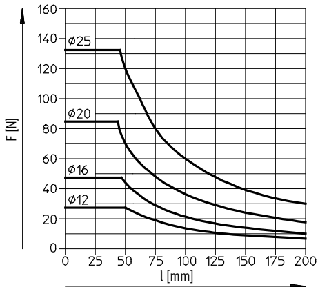
DFM-12 ... 25-GF Carrera 30 mm
