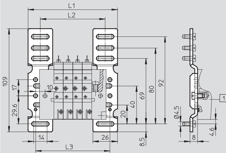
1 Ventilinsel CPV10-EX-VI
