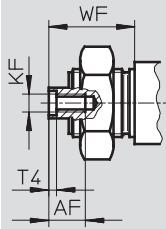
K8 – Extended piston rod
