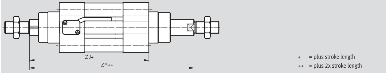
S2 / KP – Through piston rod with clamping cartridge
