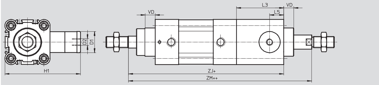
S2 / KP – Through piston rod with clamping cartridge
