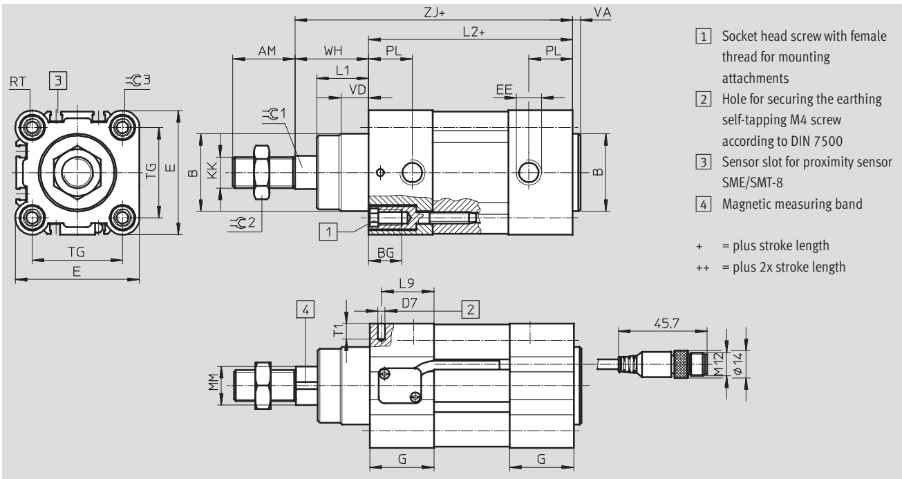
S2 – Through piston rod
