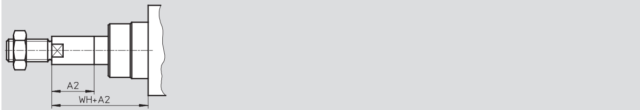
K8 – Extended piston rod
