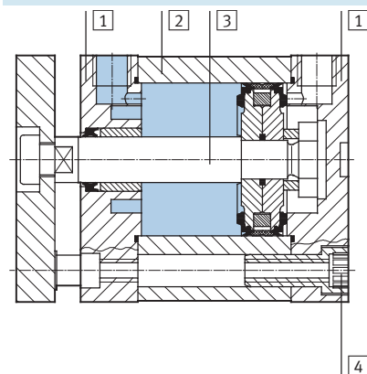
Sectional view
