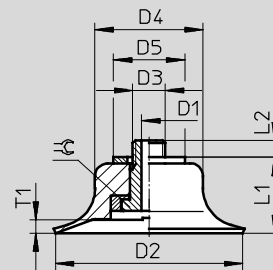
ESS-40/50/60-S
