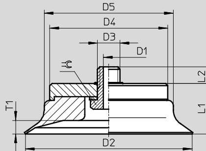
ESS-150/200-S
