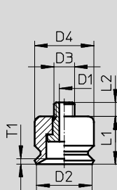
ESS-10/15-S
