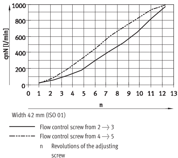
Flow rate q_N as a function of flow control
