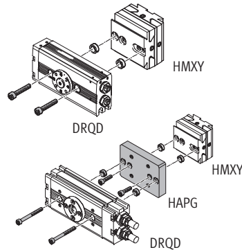
Direct mounting
