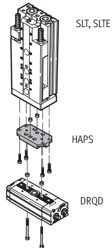
Direct mounting
