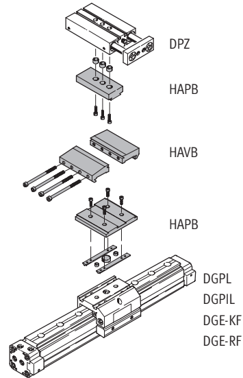
Dovetail mounting
