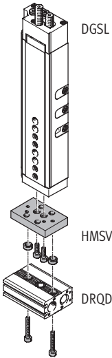
Direct mounting on yoke plate
