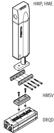
Dovetail mounting
