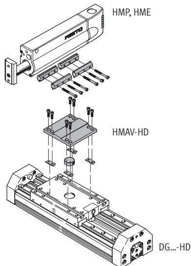
Dovetail mounting
