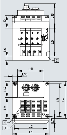
Valve terminal with installation system CPI – CPV10/14
