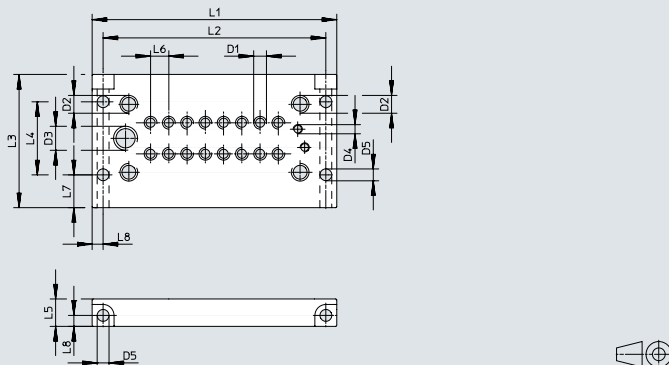
Pneumatic multiple connector plate with flange – CPV10/14/18
