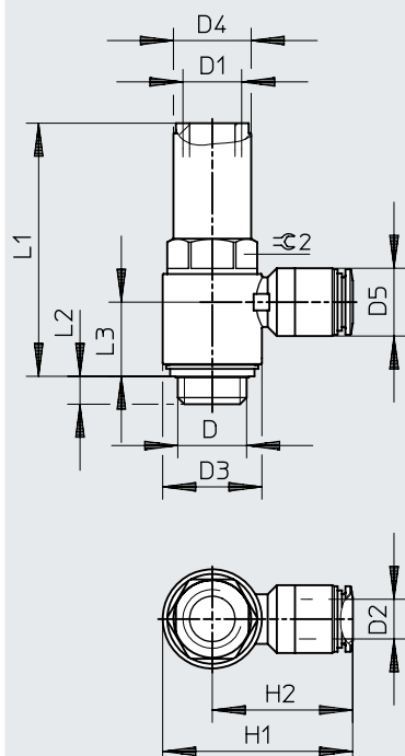
Dimensions – Push-in connector HGL-1/8, HGL-1/4, HGL-3/8
