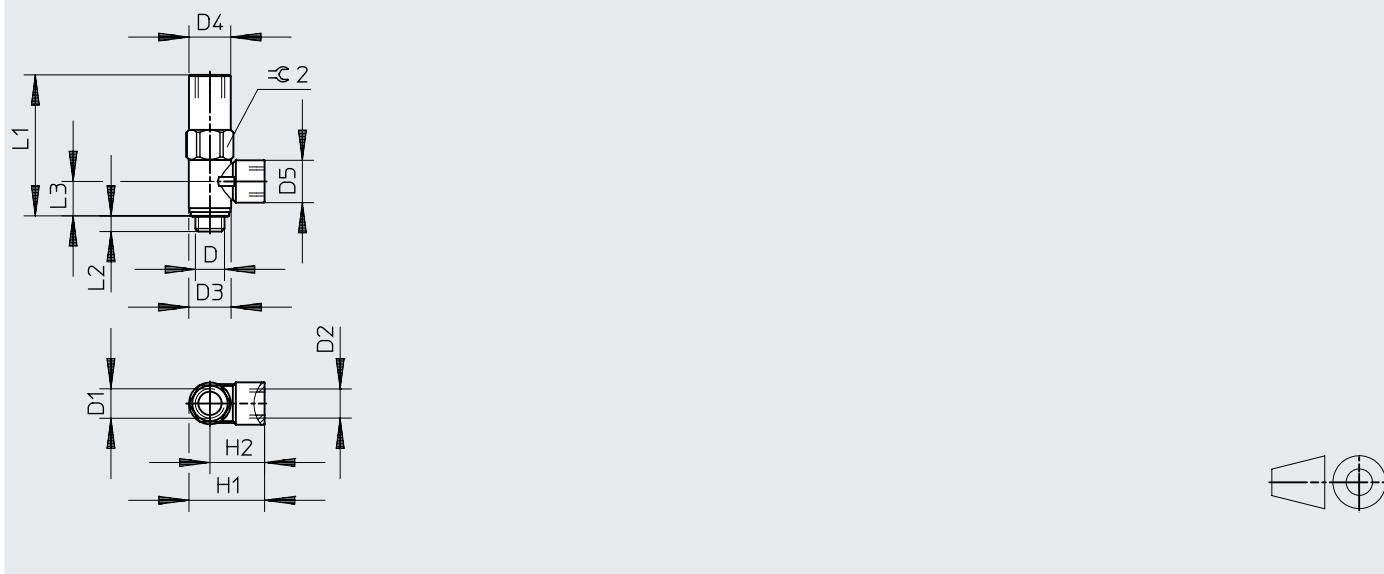
Dimensions – Female thread HGL-1/8-1/8-B
