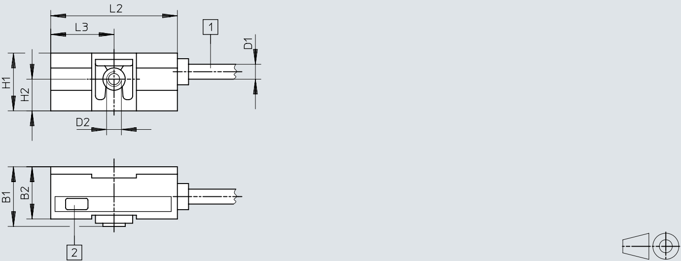
Dimensiones – SMT0-1 – Cable
