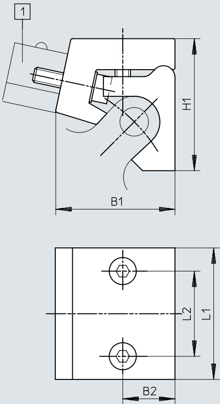
[1] Sensor de proximidad SMEO, SMT0, SMPO-1
