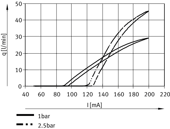
Characteristic flow rate curve, nominal width 2.2 mm, 1 bar and 2.5 bar
