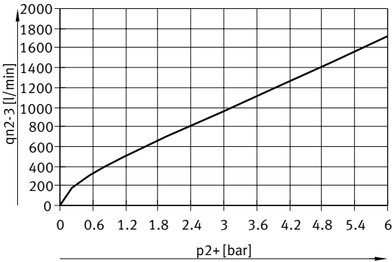
Flow rate q_n from 2 -> 3 as a function of excess output pressure p_2 , VPPM-8L/F-...-0L6H-... (6 bar)
