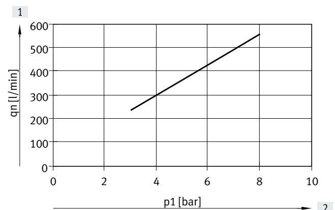
[1] Air consumption
