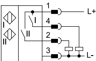
[M12] Plug M12, A-coded
