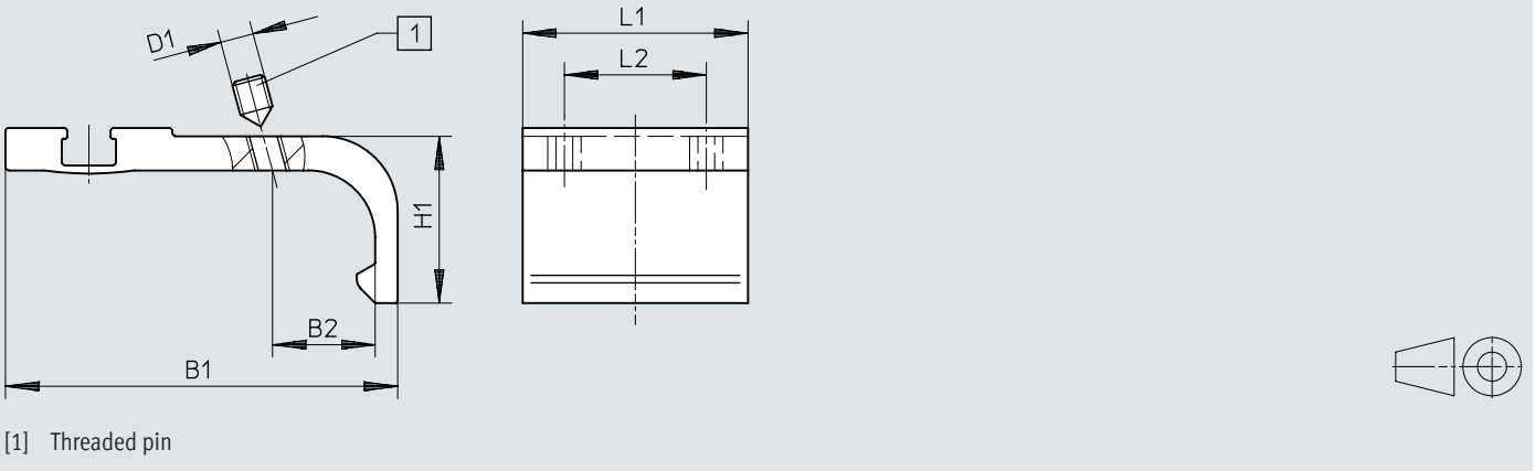
Dimensions – Mounting kit SMB-8-FENG
