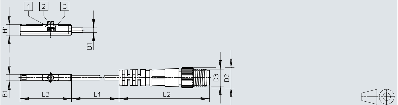
Dimensions – Proximity switch with plug
