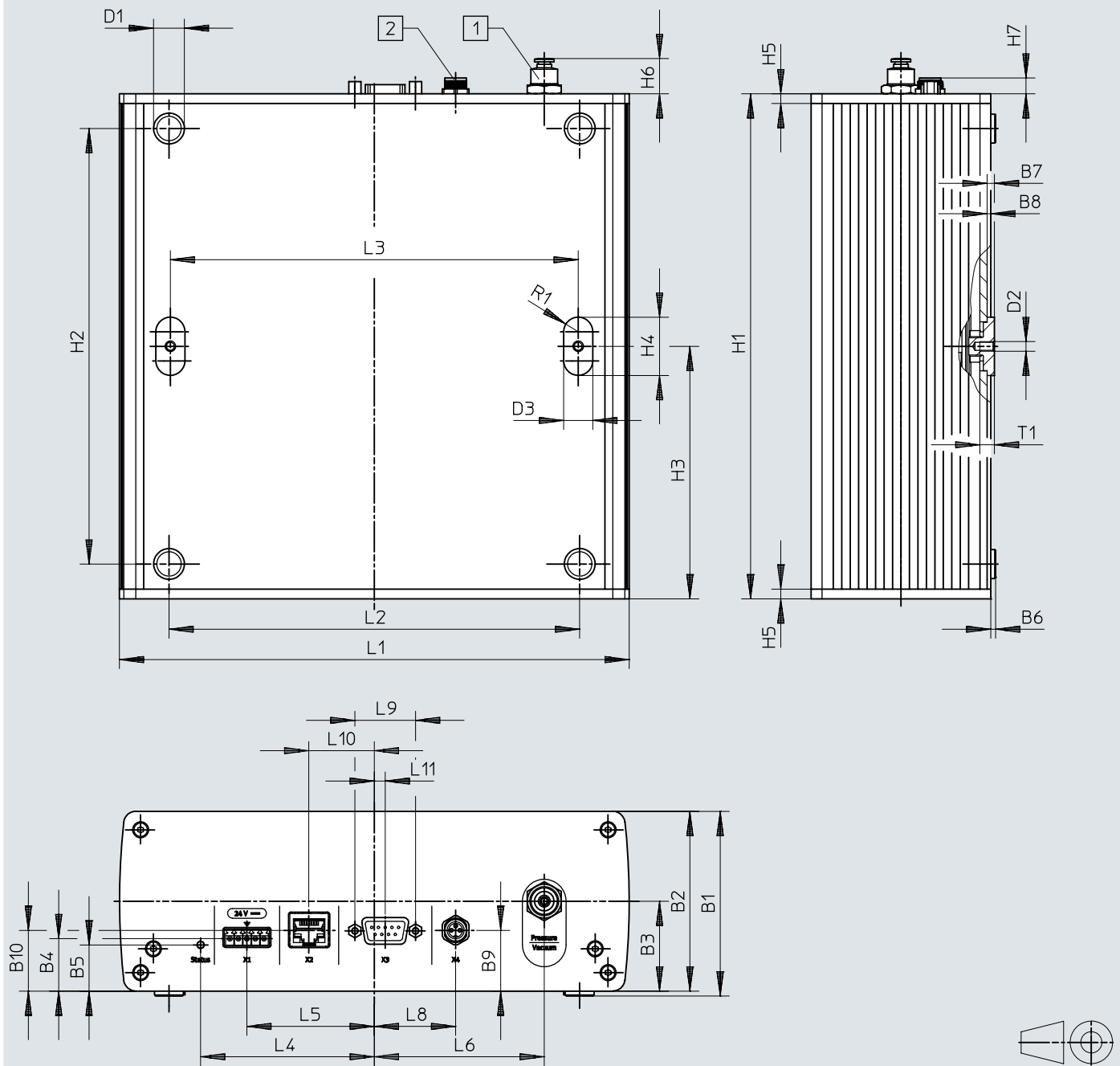
Dimensions – PGVA-1
