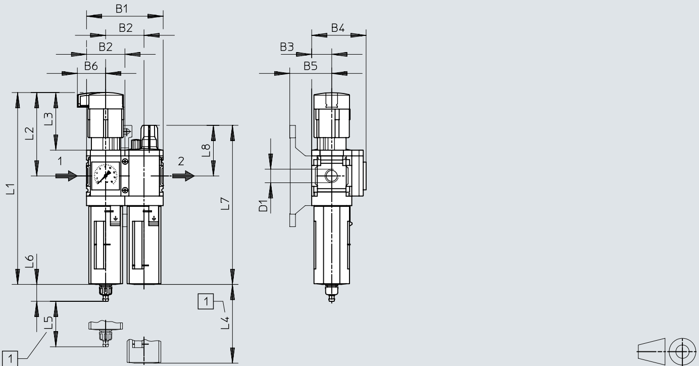
[1] Installation dimension
