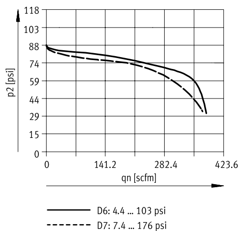
Normal flow rate q_n as a function of the outlet pressure p_2 ( p_1 = 147 psi) - MS6N-LR-1/2
