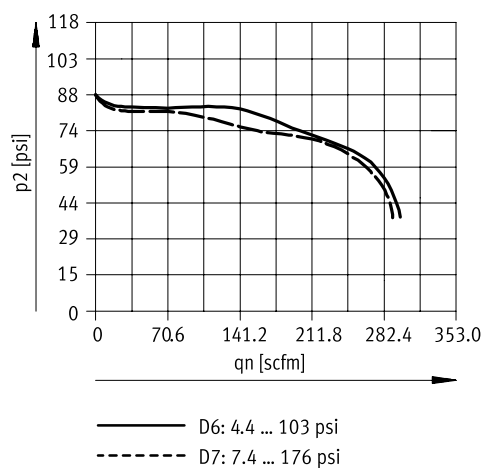
Normal flow rate q_n as a function of the outlet pressure p_2 ( p_1 = 147 psi) - MS6N-LR-3/8
