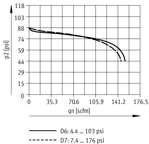
Normal flow rate q_n as a function of the outlet pressure p_2 ( p_1 = 147 psi) - MS6N-LR-1/4
