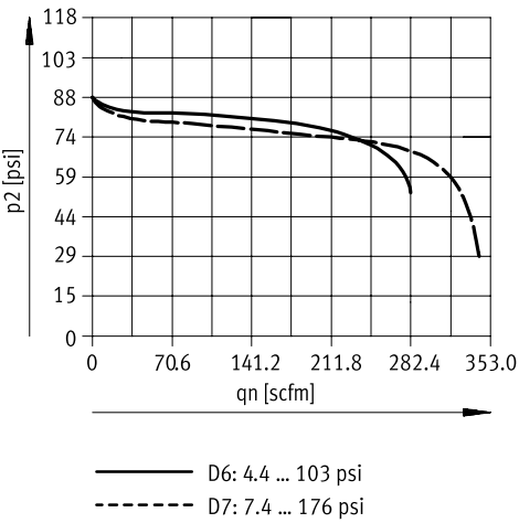
Normal flow rate qn as a function of the outlet pressure p2 (p1 = 147 psi) - MS6N-LRB-1/2
