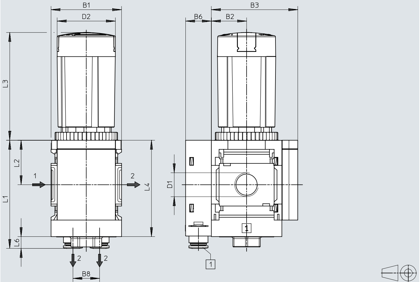
Dimensions – Angled outlet block, pressure output to rear
