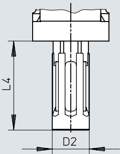
Dimensions – Silencer
