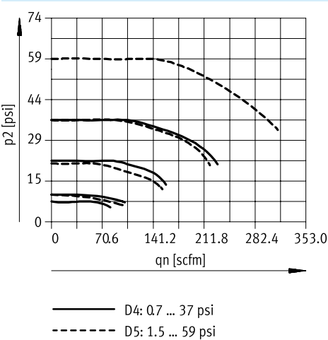
Normal flow rate q_n as a function of the outlet pressure p_2 ( p_1 = 147 psi) - MS6N-LRP-1/2
