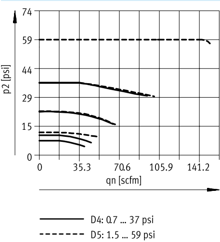
Normal flow rate q_n as a function of the outlet pressure p_2 ( p_1 = 147 psi) - MS6N-LRP-1/4
