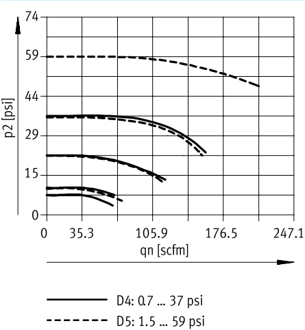
Normal flow rate q_n as a function of the outlet pressure p_2 ( p_1 = 147 psi) - MS6N-LRP-3/8
