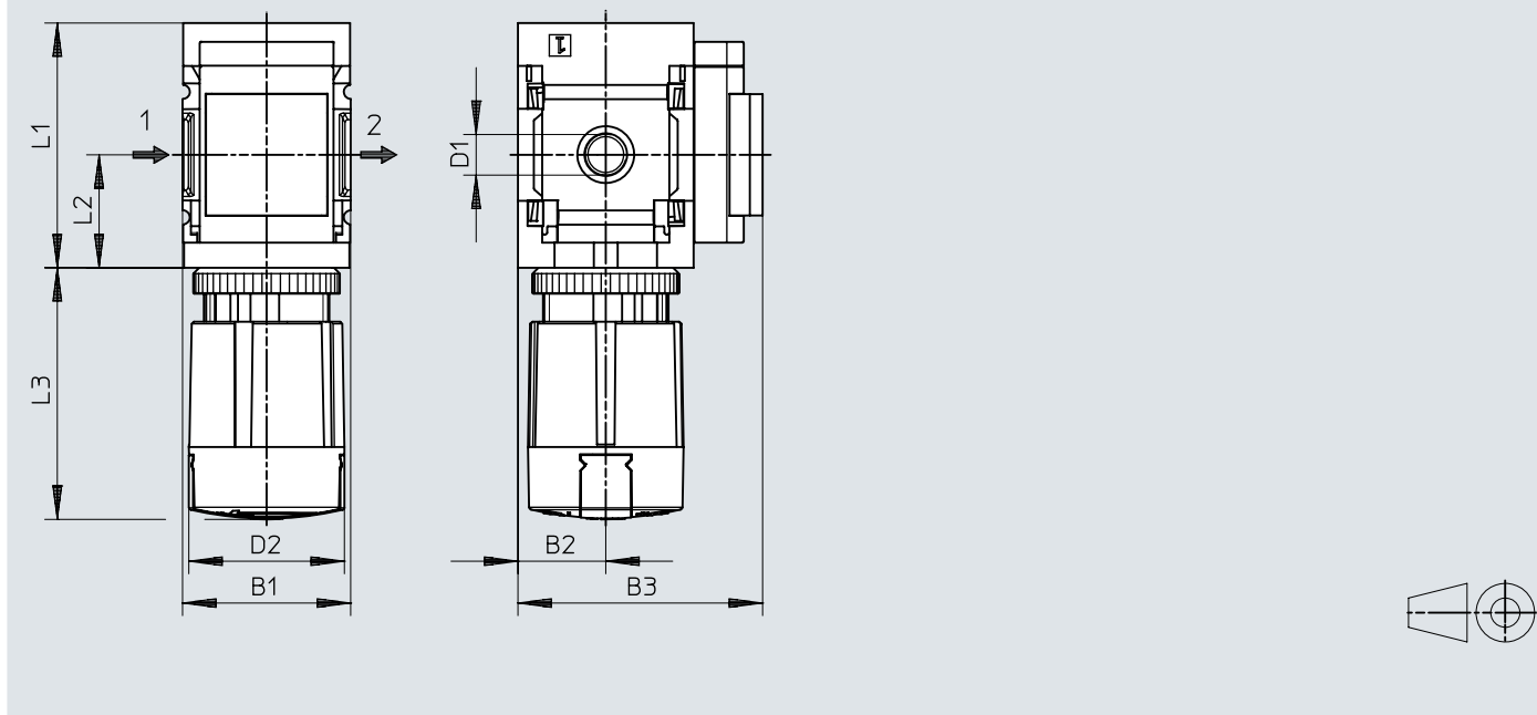
Dimensions – Alternative mounting position, rotary knob at the bottom
