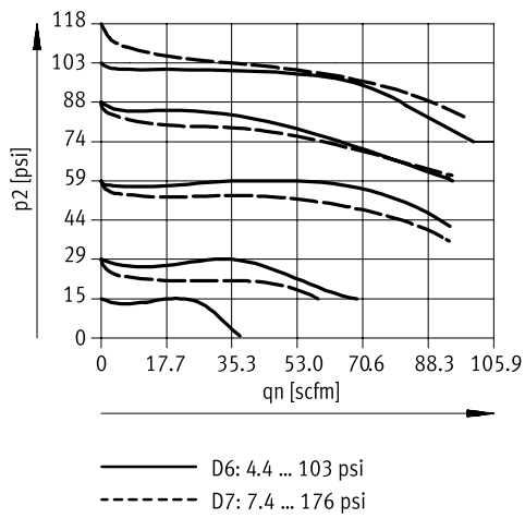
Normal flow rate q_n as a function of outlet pressure p_2 ( p_1 = 10 \text{ bar} ) - MS4-LR-1/8-D7-.. (0.5 ... 12 bar)
