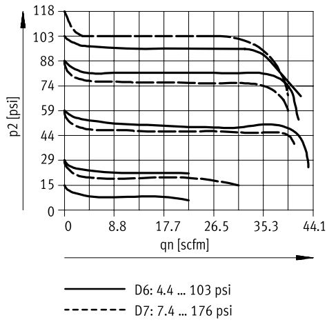
Normal flow rate q_n as a function of the outlet pressure p_2 ( p_1 = 147 \text{ psi} ) - MS4N-LR-1/8
