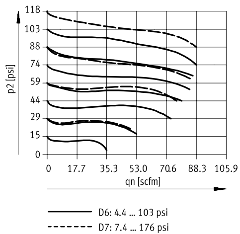
Normal flow rate q_n as a function of the outlet pressure p_2 ( p_1 = 147 psi) - MS4N-LRB-1/4
