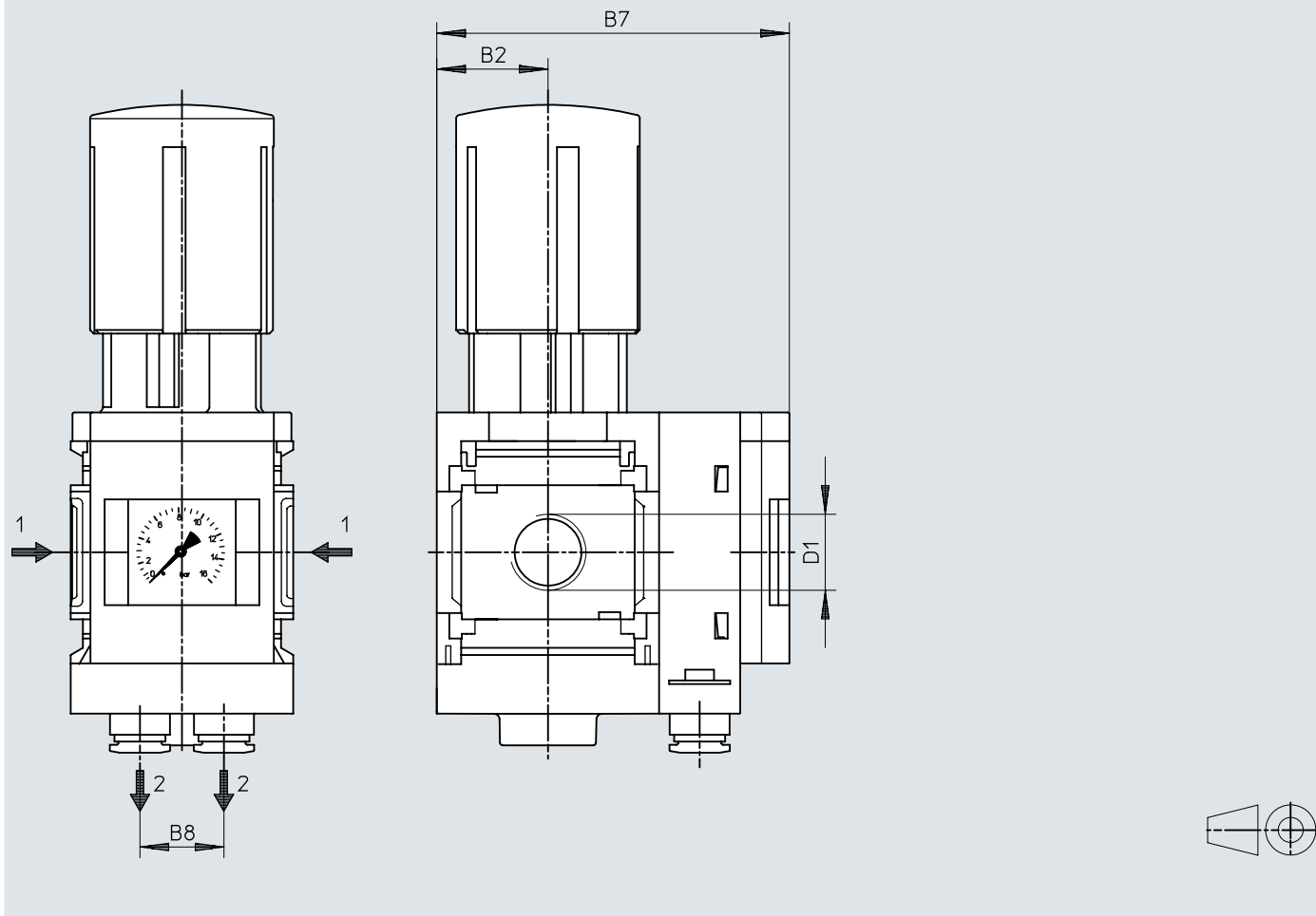
Dimensions – Angled outlet block, pressure output to front
