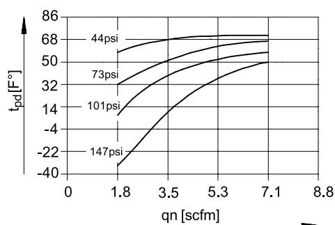
Pressure dew point t pd (outlet) as a function of the standard flow rate at outlet q n (MS4N-LDM1-...-P10)
