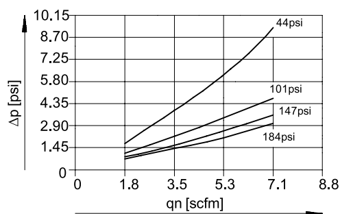
Differential pressure Δp as a function of the standard flow rate at outlet q n (MS4N-LDM1-...-P10)
