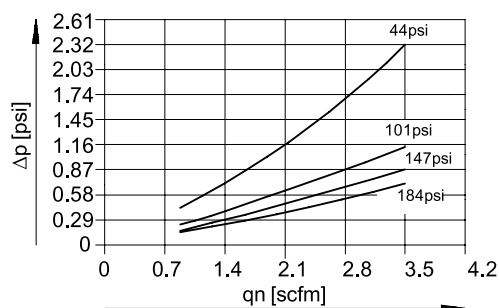
Differential pressure Δp as a function of the standard flow rate at outlet q n (MS4N-LDM1-...-P05)
