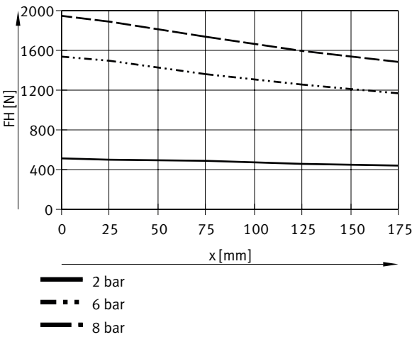
Gripping force FH per Gripper jaw as a function of the operating pressure and the Lever arm x - External gripping (closing) - HPPL-63-200
