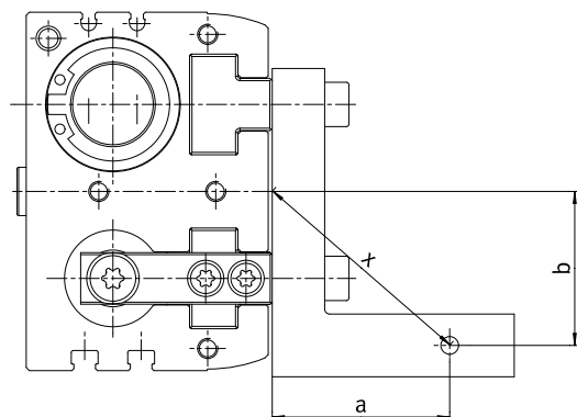
Gripping force FH per gripper jaw at 0.6 MPa (6 bar, 87 psi) as a function of lever arm x and eccentricity a and b
