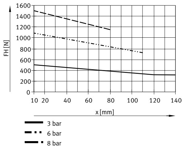
Gripping force F_H per gripper jaw as a function of operating pressure and lever arm x – internal gripping (opening), high gripping force – HGDT-63-...-F
