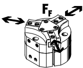
Spring force F_F as a function of size, gripper jaw stroke l and lever arm x , per gripper finger – with gripping force retention
