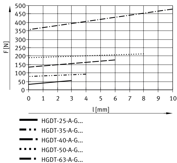
Spring force F_F as a function of the size, the gripper jaw stroke l and the lever arm x , per gripper finger – wWith gripping force retention, standard gripping force – HGDT-...-G...
