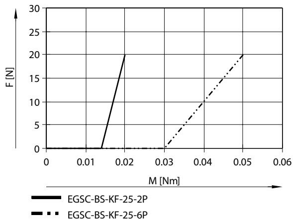
Feed force F as a function of input torque M for size 25
