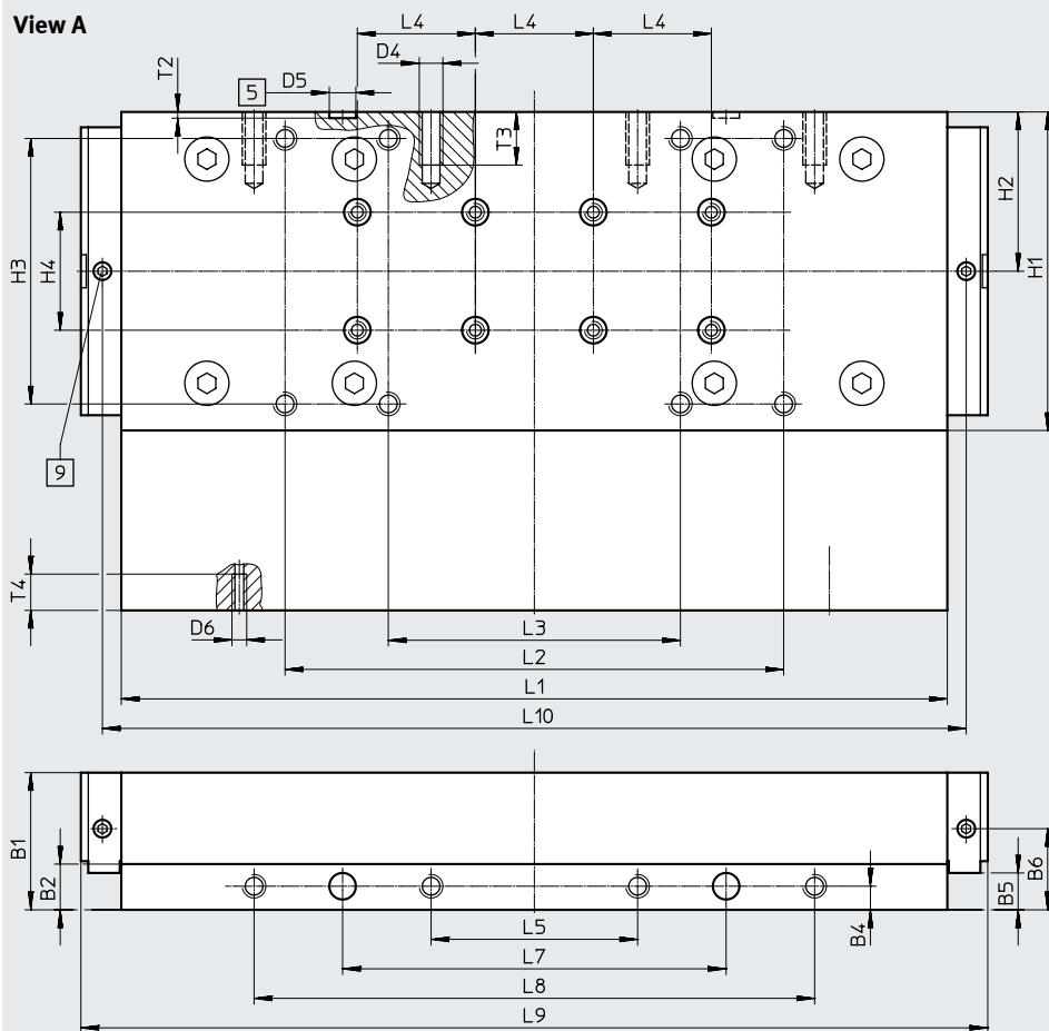
View A
