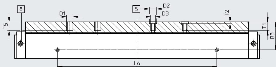
View A
