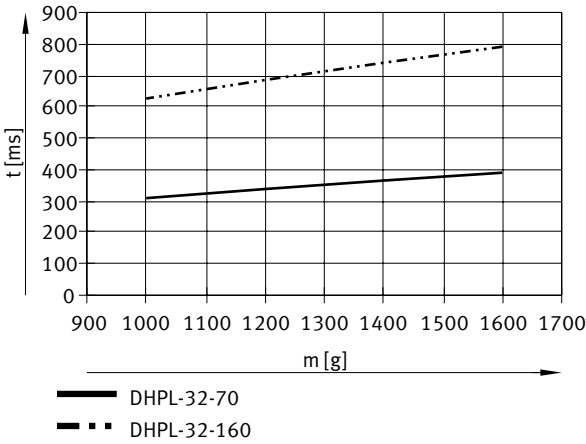
Opening and closing times as a function of gripper finger mass – DHPL-32
