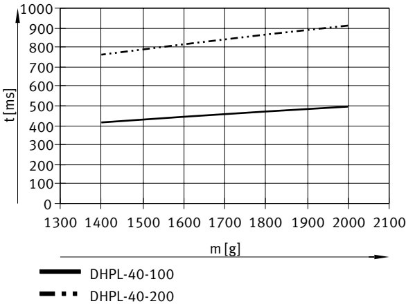
Opening and closing times as a function of gripper finger mass – DHPL-40
