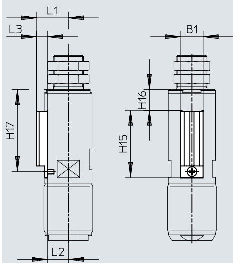
Dimensions – Sensor rail DASP-...-U
