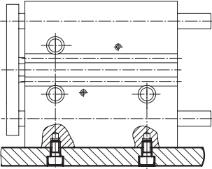
Side mounting from below
