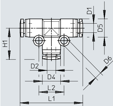
Dimensions – Push-in T-connector QBMT-...T, reducing
