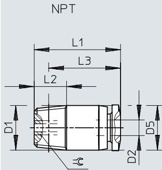
Dimensions – Push-in fitting QBM-...-I, NPT thread
