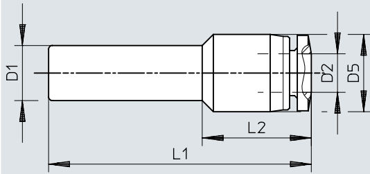
Dimensions – Push-in connector QBM-...H
