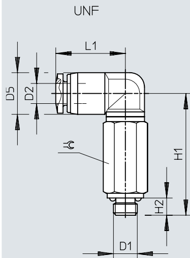
Dimensions – Push-in L-fitting, long QBMLL, UNF thread
