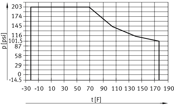
Operating pressure p as a function of temperature t (PLN; NPT)
