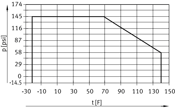
Operating pressure p as a function of temperature t (PEN; NPT)
