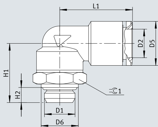
Dimensions – Push-in L-fitting NPQM-L, male thread with external hex
