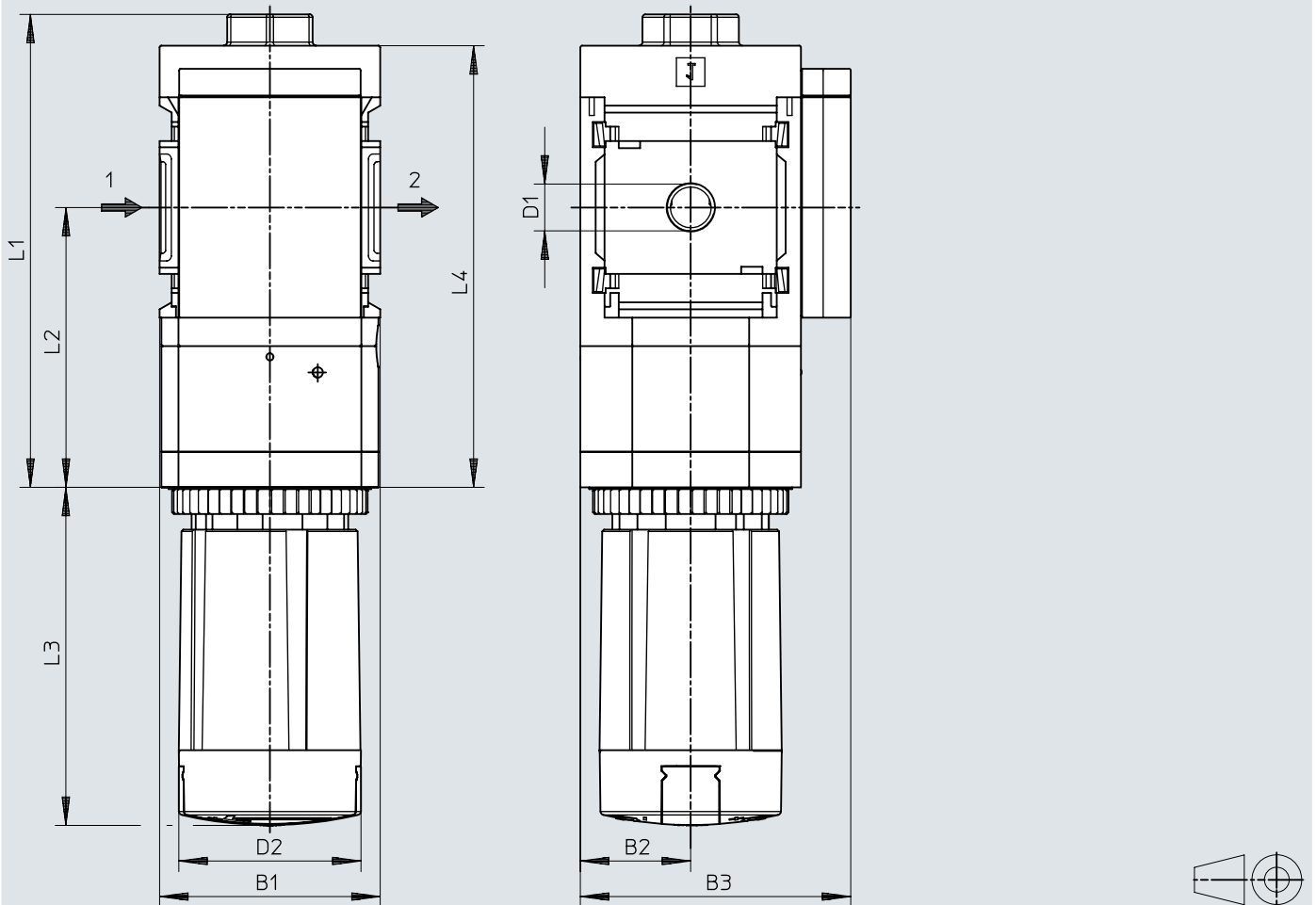
Dimensions – Alternative mounting position, rotary knob underneath
